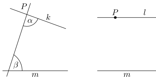
Figure 7.1 The parallel postulate
