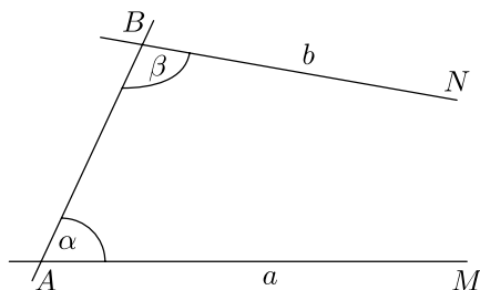
Figure 9.3 Parallels and equal angles in Bolyai's geometry
