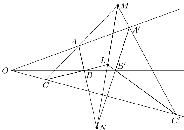
Figure 3.2 Desargues' theorem
