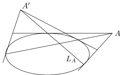
Figure 4.1 Pole and polar
