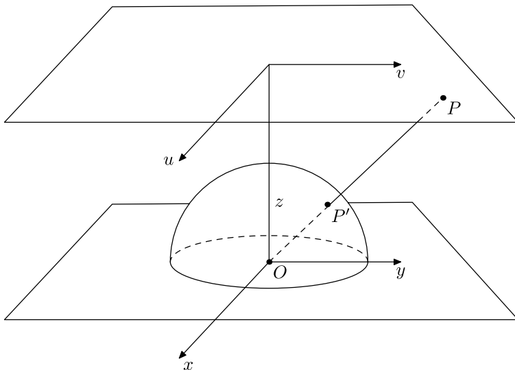
Figure 19.1 Geodetic projection (1)
