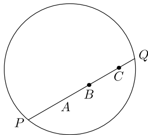
Figure 20.2 Klein's disc
