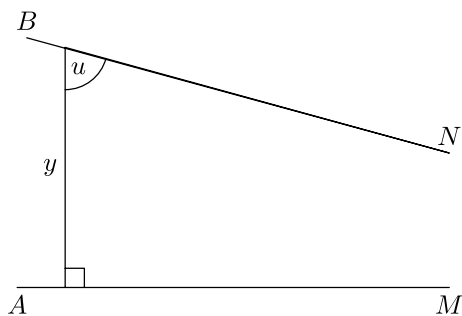
Figure 9.7 The angle of parallelism
