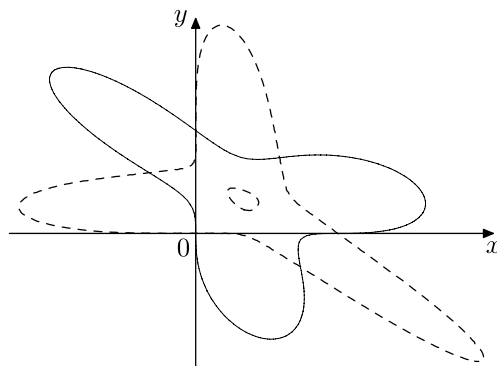
Figure 16.3 Klein's quartic curve and its Hessian
