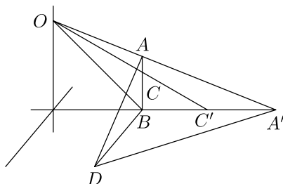
Figure 3.10 The angles \angle BAD and \angle BA'D are not equal
