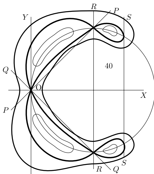
Figure 15.1 Plücker's quartic
