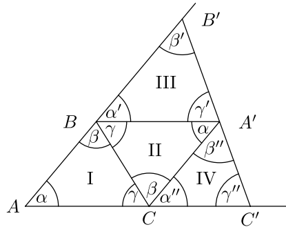
Figure 7.3 Legendre's figure
