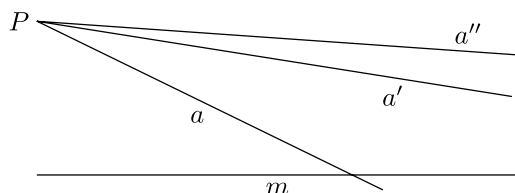
Figure 9.1 A parallel line as a limiting case
