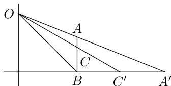
Figure 3.9 The ratios AC/CB and A'C'/C'B are not equal
