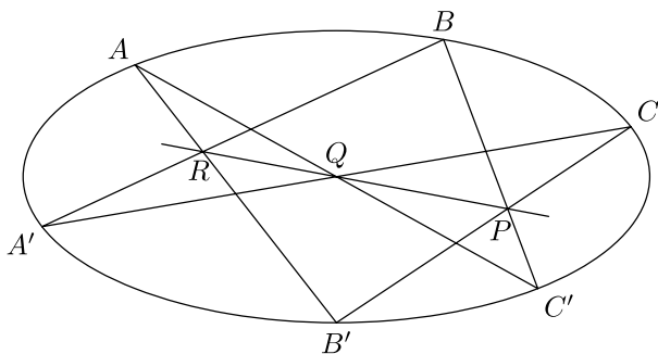
Figure 3.3 Pascal's theorem
