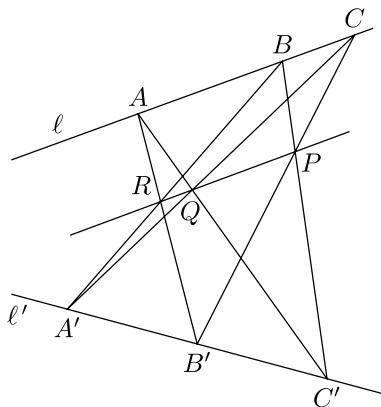
Figure 3.1 Pappus's theorem
