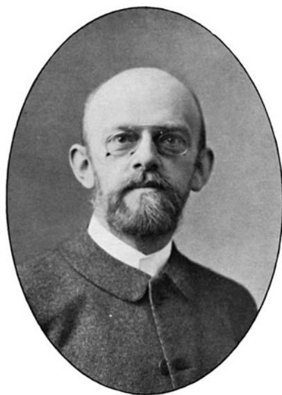
Figure 23.1 Hilbert
