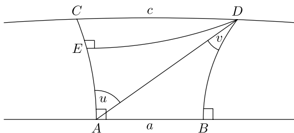
Figure 9.9 The angles u and v
