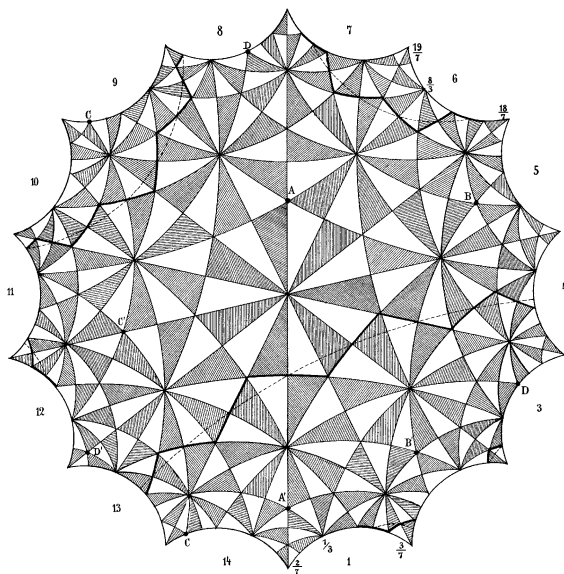
Figure 25.3 The tessellation (2, 3, 7)
