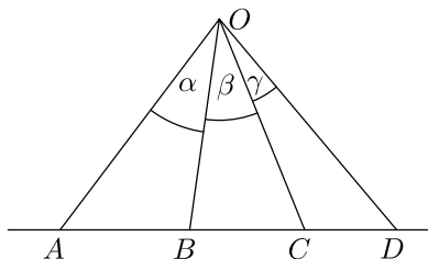
Figure 6.2 Cross-ratio in terms of angles
