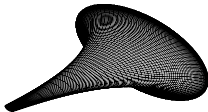
Figure 11.1 A pseudosphere
