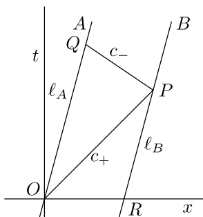
Figure 29.1 Changing coordinates
