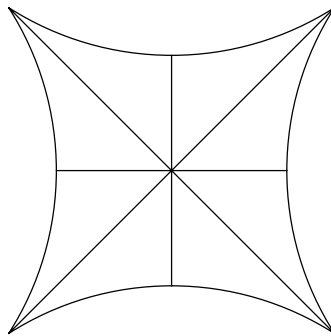
Figure 8.2 Schweikart's square
