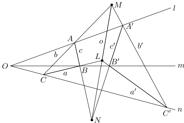
Figure 5.2 Desargues' dual
