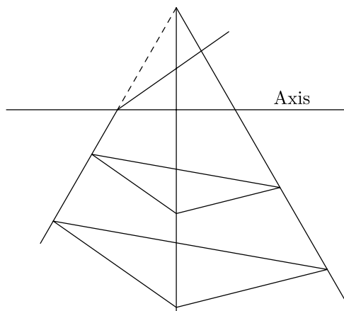
Figure 23.3 The failure of Desargues' theorem
