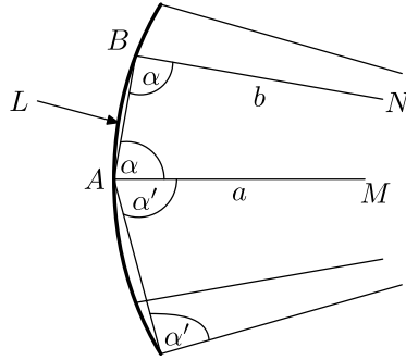
Figure 9.4 Bolyai's L -curve
