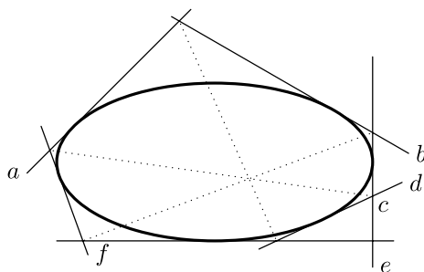
Figure 5.3 Brianchon's theorem
