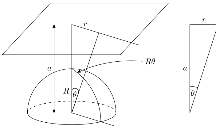
Figure 19.2 Geodetic projection (2)
