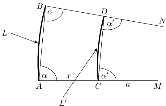
Figure 9.8 The curve L'
